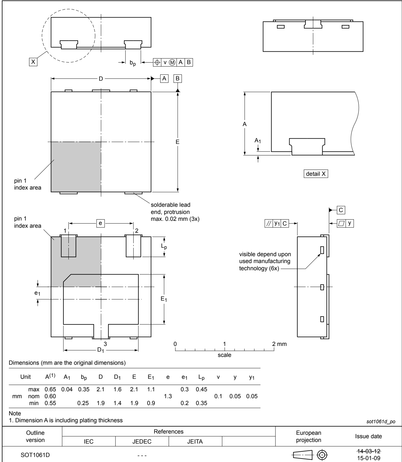
Fig. 1. Package outline DFN2020D-3 (SOT1061D)
